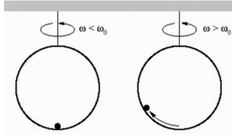
Fig. 1.51. The ball in the hoop system: left–stable, right–unstable (adapted from [Mar99]).
