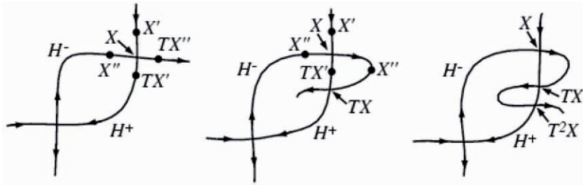
Fig. 1.28. More on homoclinic tangle (see text for explanation).
