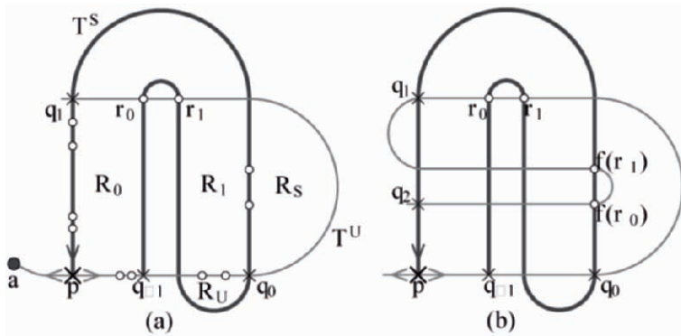
Fig. 2.3. The full horseshoe trellis: (a) with signature 2; (b) with signature 3 (adapted from [Col02, Col05]).
