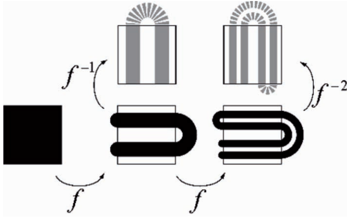
Fig. 1.23. Iterated horseshoe map: pre-images of the square region.
