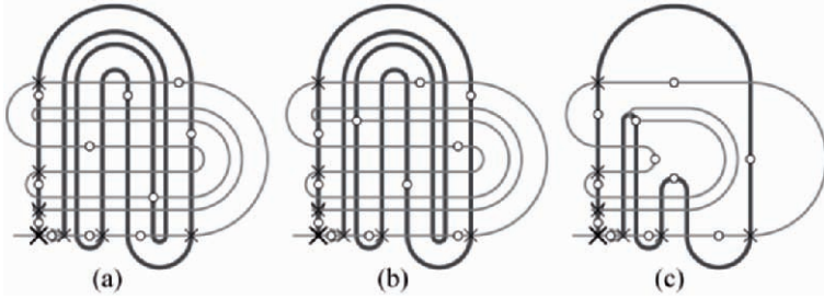
Fig. 2.8. The horseshoe trellis and homoclinic orbits with codes (a) \bar{0}110111\bar{0} and (b) \bar{0}111011\bar{0} , and (c) the trellis they force (adapted from [Col02, Col05]).
