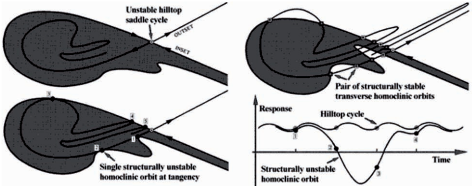
Fig. 1.27. Dynamics of a homoclinic tangle. The hill-top solution of a damped particle in a potential well driven by a periodic force. As the driving increases, the inset and outset get tangled.
