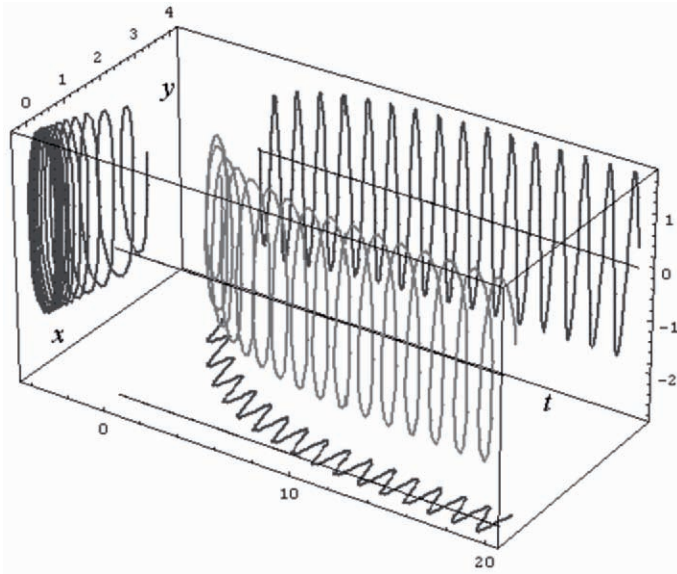
Fig. 1.10. Time-phase plot of the forced Rayleigh's self-sustained oscillator with the following parameters: A = 1.3 , B = 1.5 , C = 0.7 , L = 1.5 , x_0 = 3 , y_0 = 0 , t_{max} = 20 s, F = 10 , w = 5 . Simulated using Mathematica TM .
