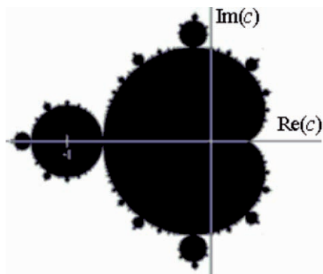
Fig. 7.1. The Mandelbrot set in a complex plane.
