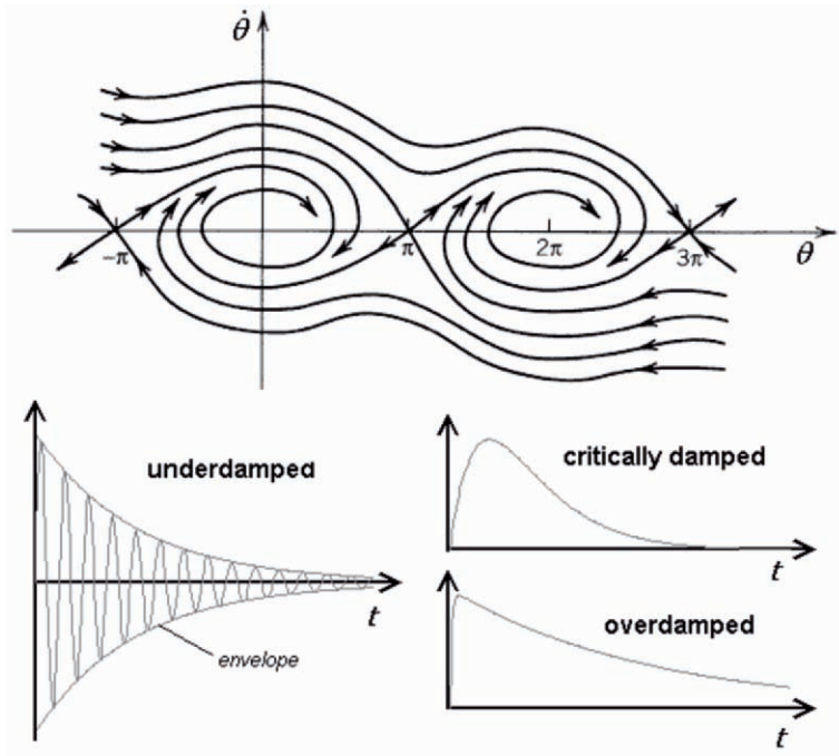
Fig. 1.38. A damped gravity pendulum settles to a rest: its phase portrait (up) shows spiralling orbits that lead to a focus attractor; its time plot (down) shows three common damping cases.
