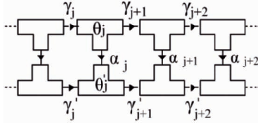
Fig. 6.2. Josephson junction Ladder (JLJ).
