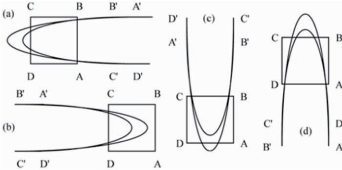
Fig. 2.9. The Hénon-like map of degree 2 (adapted from [Obe87, Obe00]).
