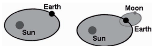
Fig. 1.17. The 2-body, problem solved by Newton (left), and the 3-body problem, first attacked by Poincaré, and still the point of active research (right).
