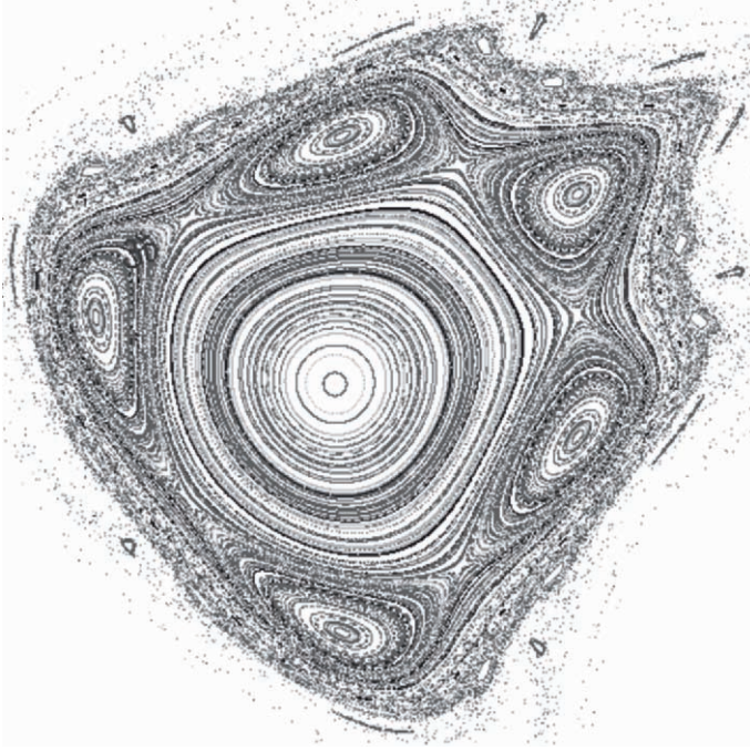
Fig. 1.35. Phase-plot of the area-preserving generalized Hénon map , simulated using Dynamics Solver TM .
