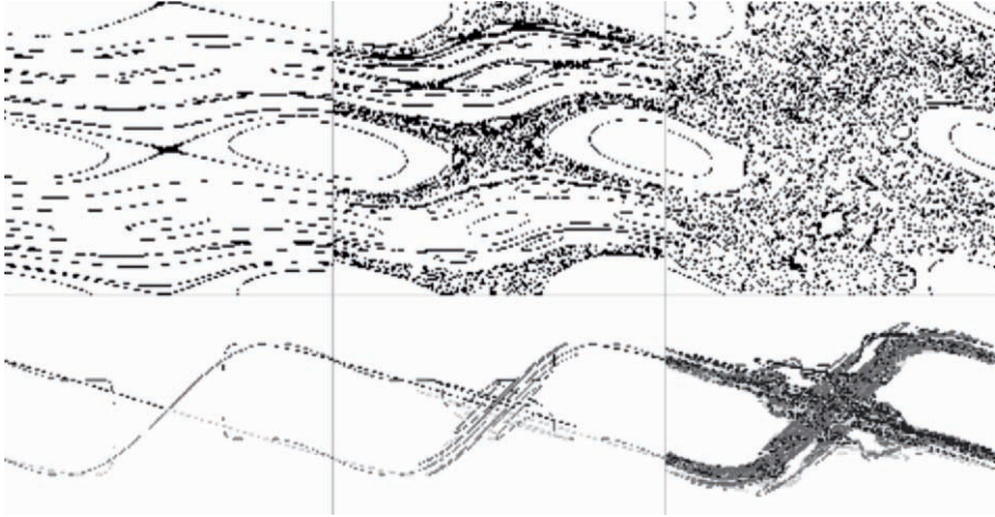
Fig. 1.58. Standard Map: Upper left: 20 trajectories with \mu = 0.08 ; the angle \varphi \in [0, 2\pi] is plotted along the horizontal, the variable r \in [0, 2] – along the vertical axis. Upper middle: the same for \mu = 0.15 . Upper right: the same for \mu = 0.25 . Lower left: beginning of the stable manifold (going from lower-left to upper-right) and unstable manifold (going from upper-left to lower-right) of the hyperbolic point (\varphi, r) = (9\pi, 1) for \mu = 0.25 . Lower middle: the same continued for two more iterations. Lower right: the same for additional 9 iterations (adapted from [Ric01]).
