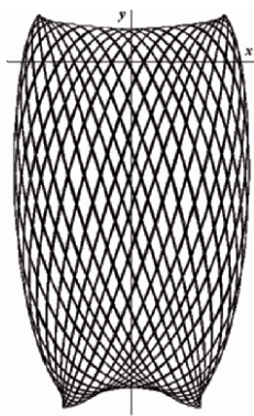
Fig. 1.46. Phase-portrait of an elastic pendulum showing Lissajous curves ; simulated using Dynamics Solver TM .
