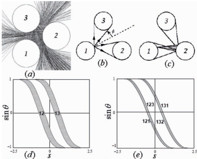
Fig. 1.16. A 3-disk pinball game. Up: (a) Elastic scattering around three hard disks (simulated in Dynamics Solver TM ); (b) A trajectory starting out from disk 1 can either hit another disk or escape; (c) Hitting two disks in a sequence requires a much sharper aim; the cones of initial conditions that hit more and more consecutive disks are nested within each other. Down: Poincaré section for the 3-disk pinball game, with trajectories emanating from the disk 1 with x_0 = (\text{arc-length}, \text{parallel momentum}) = (s_0, p_0) , disk radius: center separation ratio a : R = 1 : 2.5 ; (d) Strips of initial points M_{12}, M_{13} which reach disks 2, 3 in one bounce, respectively. (e) Strips of initial points M_{121}, M_{131}, M_{132} and M_{123} which reach disks 1, 2, 3 in two bounces, respectively; the Poincaré sections for trajectories originating on the other two disks are obtained by the appropriate relabelling of the strips (modified and adapted from [CAM05]).
