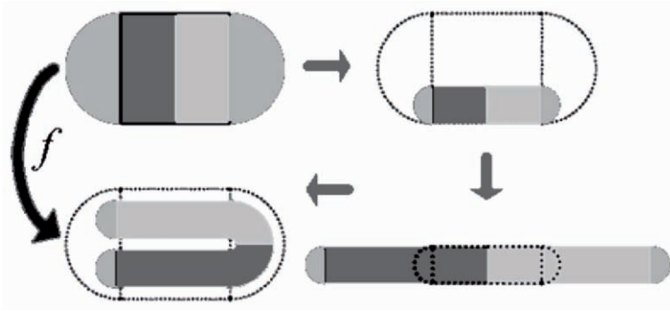
Fig. 1.21. The Smale horseshoe map f , defined by stretching, folding and squeezing of the system's phase-space.
