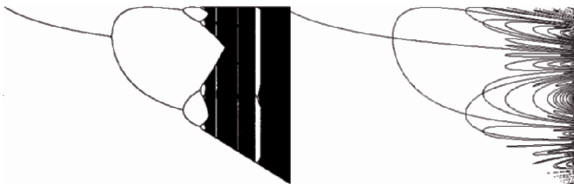
Fig. 1.30. Feigenbaum constant: approaching chaos via successive period doubling bifurcations. The plot on the left is made by iterating equation f(x) = 1 - \mu|x|^r with r = 2 several hundred times for a series of discrete but closely spaced values of \mu , discarding the first hundred or so points before the iteration has settled down to its fixed-points, and then plotting the points remaining. The plot on the right more directly shows the cycle may be constructed by plotting function f^n(x) - x as a function of \mu , showing the resulting curves for n = 1, 2, 4 . Simulated in Mathematica TM .
