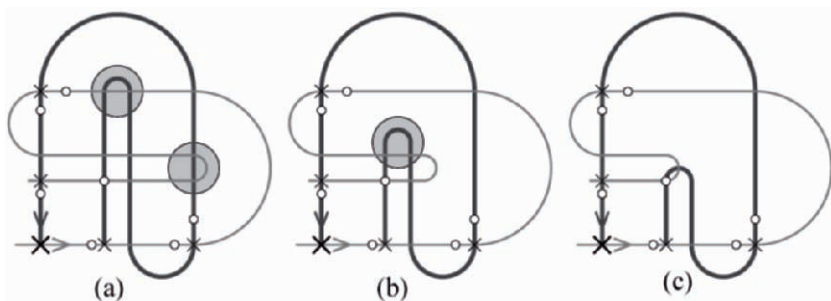
Fig. 2.4. Pruning away bigons in the horseshoe trellis (adapted from [Col02, Col05]).
