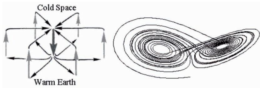
Fig. 1.29. Bénard cells, showing a typical vortex of a rolling air, with a warm air rising in a ring and a cool air descending in the center (left). A simple model of the Bénard cells provided by the celebrated ‘Lorenz–butterfly’ (or, ‘Lorenz–mask’) strange attractor (right).
