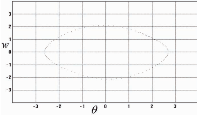
Fig. 1.4. The limit-cycle attractor in the phase portrait of the driven nonlinear pendulum.
