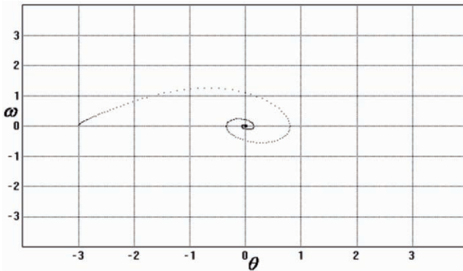
Fig. 1.3. Another phase portrait of the driven nonlinear pendulum with different initial conditions.
