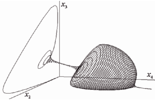
Fig. 1.47. 3D phase-portrait of the 4D autocatalator system, simulated using Dynamics Solver TM .
