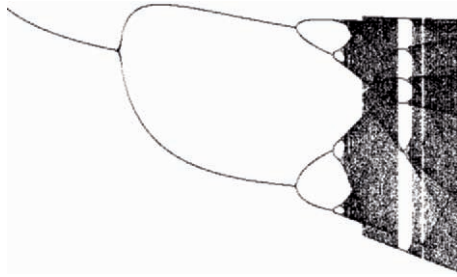
Fig. 1.33. Bifurcation diagram of the Hénon strange attractor , simulated using Dynamics Solver TM .
