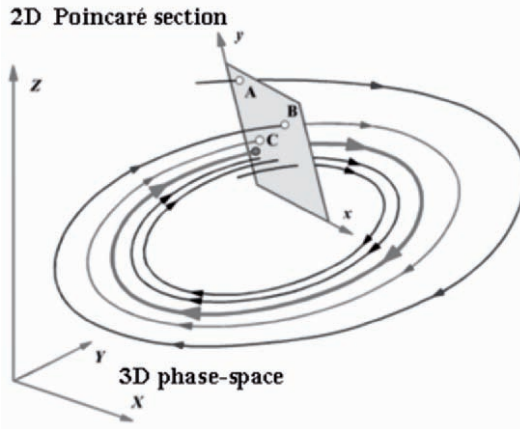
Fig. 1.18. The 2D Poincaré section, reducing the 3D phase-space, using the iterated map: x_{new} = F(x, y) , y_{new} = G(x, y) .
