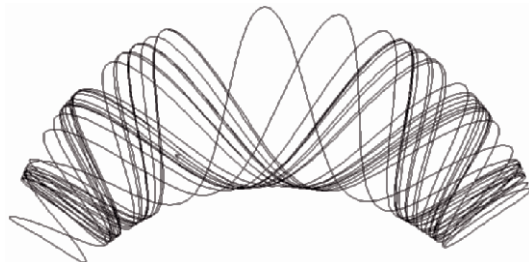
Fig. 1.45. Duffing strange attractor, showing stroboscopic Poincaré sections; simulated using Dynamics Solver TM .
