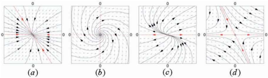
Fig. 1.54. Several examples of linear vector-fields, generated in Mathematica TM : (a) stable node, (b) unstable focus, (c) unstable node, and (d) saddle (unstable).
