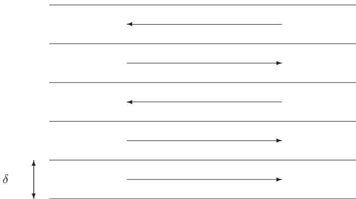
Fig. 8.3. Random shear of \pm v_0 velocity in strips of size \delta (adapted from [BLV01])
