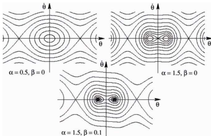
Fig. 1.52. The phase portrait for the ball in the hoop before and after the onset of instability for the case g/R = 1 (adapted from [Mar99]).
