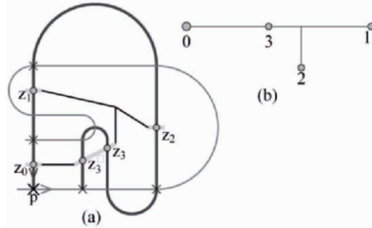
Fig. 2.5. (a) The restricted tree representative of the trellis of signature 3 forced by \bar{0}1111\bar{0} . (b) The topological tree representative of the orbit (adapted from [Col02, Col05]).
