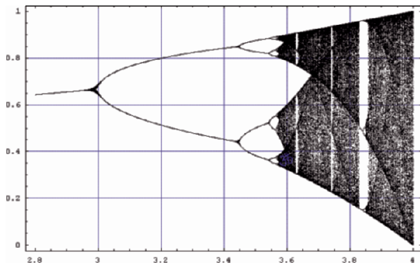
Fig. 1.31. Bifurcation diagram for the logistic map, simulated using Mathematica TM .
