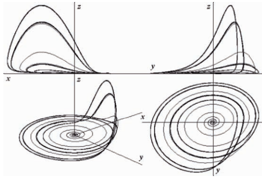
Fig. 1.42. The celebrated Rossler attractor, simulated using Dynamics Solver TM .
