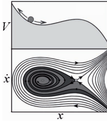
Fig. 1.26. Motion of a damped particle in a potential well, driven by a periodic force F \cos(\omega t) . Up: potential (x - V) -plot, with V = x^2/2 - x^3/3 ; down: the corresponding phase (x - \dot{x}) -portrait, showing the safe basin of attraction – if the driving is switched off ( F = 0 ).
