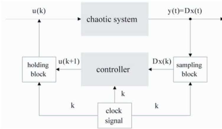
Fig. 7.5. Block-diagram for the chaos-control system (adapted from [YC98]).
