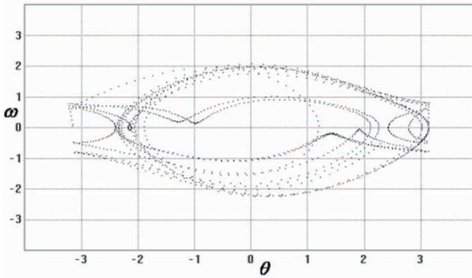
Fig. 1.5. Chaotic phase portrait of the driven nonlinear pendulum.
