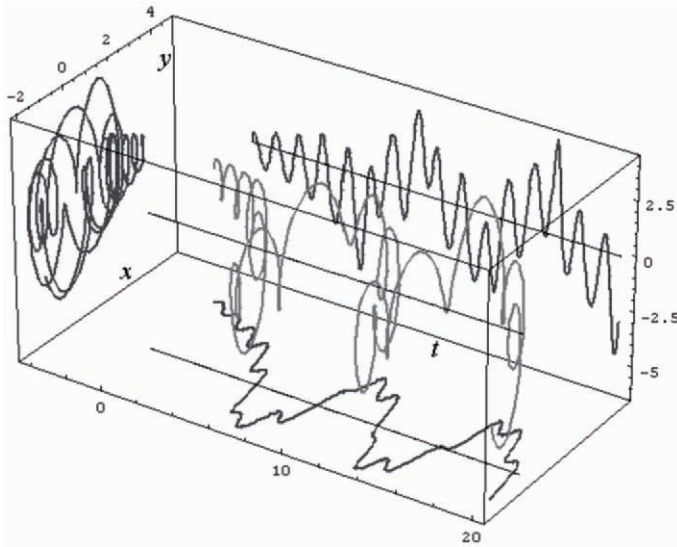
Fig. 1.12. Time-phase plot of the forced Van der Pol oscillator with the following parameters: A = 1.3 , B = 1.5 , C = 0.7 , L = 1.5 , x_0 = 3 , y_0 = 0 , t_{max} = 20 s, F = 10 , w = 5 . Simulated using Mathematica TM .
