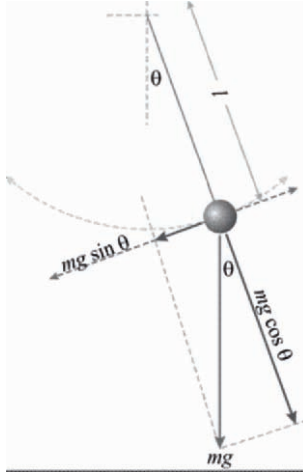
Fig. 1.36. Force diagram of a simple gravity pendulum.
