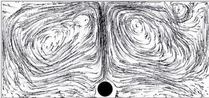
Fig. 8.5. An example of trajectories obtained by PTV technique in the convective cell at Ra = 2.39 \times 10^8 . The vertical thermal plume is clearly observable. The dark circle on the bottom represents the heat source.
