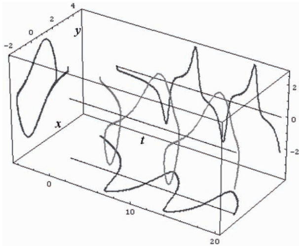
Fig. 1.11. Time-phase plot of the free Van der Pol oscillator with the following parameters: A = 1.3 , B = 1.5 , C = 0.7 , L = 1.5 , x_0 = 3 , y_0 = 0 , t_{max} = 20 s. Simulated using Mathematica TM .
