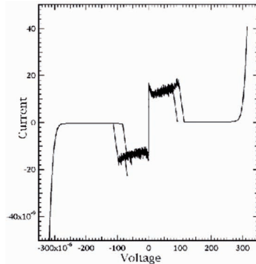
Fig. 6.1. Josephson junction: the current–voltage curve obtained at low temperature. The vertical portions (zero voltage) of the curve represent Cooper pair tunnelling. There is a small magnetic field applied, so that the maximum Josephson current is severely reduced. Hysteresis is clearly visible around 100 microvolts. The portion of the curve between 100 and 300 microvolts is current independent, and is the regime where the device can be used as a detector.
