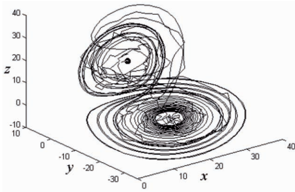
Fig. 3.2. Nonlinear control of the Lorenz system: targeting of unstable upper and lower states in the Lorenz attractor (after applying random perturbations, see [Pet96]), using a MIMO nonlinear controller (see [II06b]); simulated using Matlab TM .
