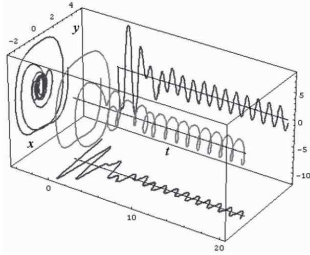
Fig. 1.8. Time-phase plot of the forced hard spring with the following parameters: m = 0.5 \text{ kg} , a = 1.3 , b = 0.7 , c = 0.5 , x_0 = 3 , y_0 = 0 , t_{max} = 20 \text{ s} , F = 10 , w = 5 . Simulated using Mathematica TM .
