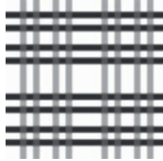
Fig. 1.24. Intersections that converge to the invariant set A .
