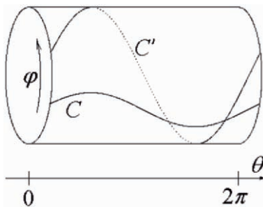
Fig. 7.3. Torus unwrapped in the \theta direction. The map (7.5) takes the curve C to the curve C' (adapted and modified from [KKH03]).
