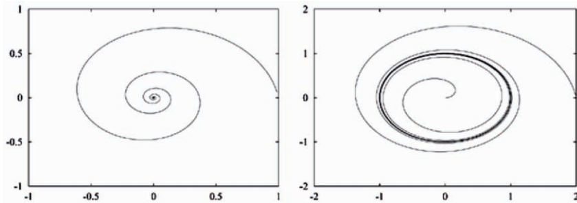
Fig. 1.14. Examples of regular attractors: fixed-point (left) and limit cycle (right). Note that limit cycles exist only in nonlinear dynamics.
