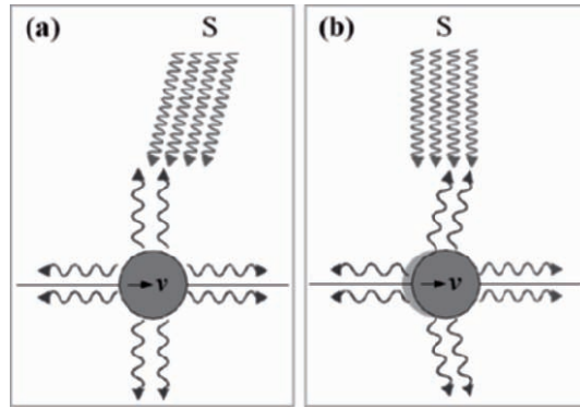
Fig. 3.1. Poynting–Robertson (PR) effect: radiation from the Sun (S) and thermal radiation from a particle seen (a) from an observer moving with the particle; and (b) from an observer at rest with respect to the Sun.
