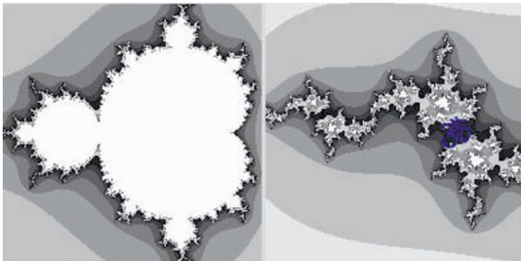
Fig. 1.48. The celebrated conformal Mandelbrot (left) and Julia (right) sets in the complex plane, simulated using Dynamics Solver TM .
