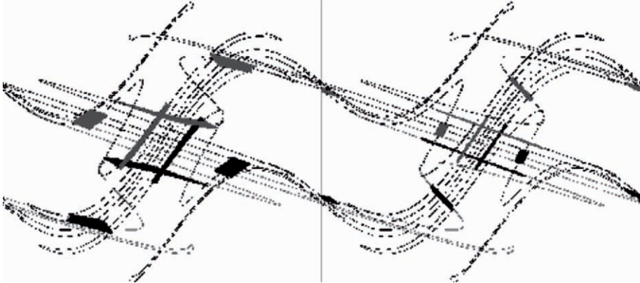
Fig. 1.59. Smale horseshoe in the standard map for \mu = 0.4 ; the angle \varphi \in [0, 2\pi] is plotted along the horizontal, the variable r \in [0, 2] – along the vertical axis. Left: the intersection of the two pairs of strips near the center contains an invariant set for M^3 . Right: the same for M^4 (adapted from [Ric01]).
