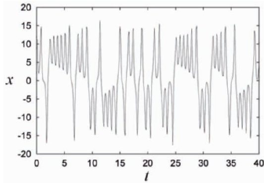
Fig. 1.15. Example of an aperiodic signal: the x variable of the Lorenz system (1.7) as function of time t , for r = 28 .
