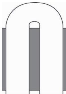
Fig. 1.20. The Smale horseshoe map consists of a sequence of operations on the unit square. First, stretch in the y -direction by more than a factor of two, then squeeze (compress) in the x -direction by more than a factor of two. Finally, fold the resulting rectangle and fit it back onto the square, overlapping at the top and bottom, and not quite reaching the ends to the left and right (and with a gap in the middle), as illustrated in the diagram. The shape of the stretched and folded map gives the horseshoe map its name. Note that it is vital to the construction process for the map to overlap and leave the middle and vertical edges of the initial unit square uncovered.
