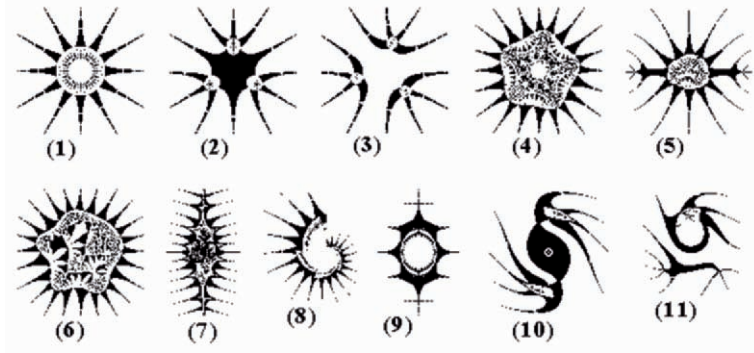
Fig. 1.50. Pickover's biomorphs (see text for details).
