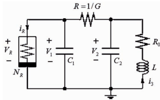
Fig. 1.43. Chua's circuit.
