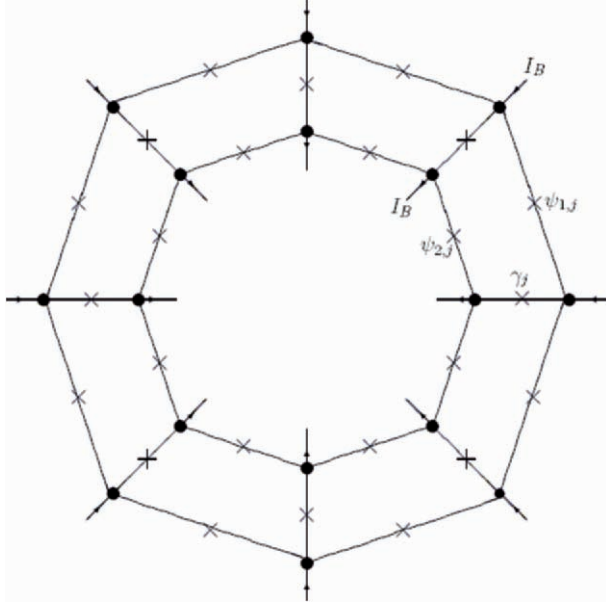
Fig. 6.3. A ladder array of Josephson junctions with periodic boundary conditions and N = 8 plaquettes. A uniform, dc bias current I_B is inserted into and extracted from each rung as shown. The gauge-invariant phase difference across the rung junctions is denoted by \gamma_j where 1 \leq j \leq N , while the corresponding quantities for the off-rung junctions along the outer(inner) edge are \psi_{1,j}(\psi_{2,j}) (adapted and modified from [TSS05]).
