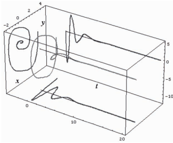
Fig. 1.7. Time-phase plot of the free hard spring with the following parameters: m = 0.5 \text{ kg} , a = 1.3 , b = 0.7 , c = 0.5 , x_0 = 3 , y_0 = 0 , t_{max} = 20 \text{ s} . Simulated using Mathematica TM .
