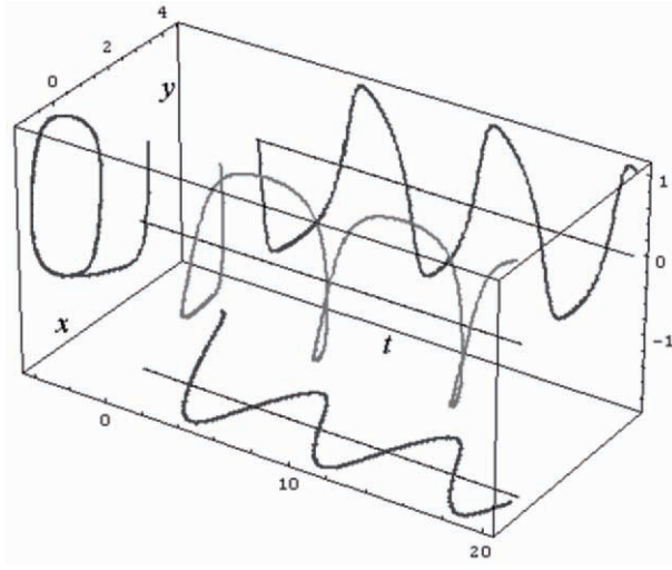
Fig. 1.9. Time-phase plot of the free Rayleigh's self-sustained oscillator with the following parameters: A = 1.3 , B = 1.5 , C = 0.7 , L = 1.5 , x_0 = 3 , y_0 = 0 , t_{max} = 20 s. Simulated using Mathematica TM .
