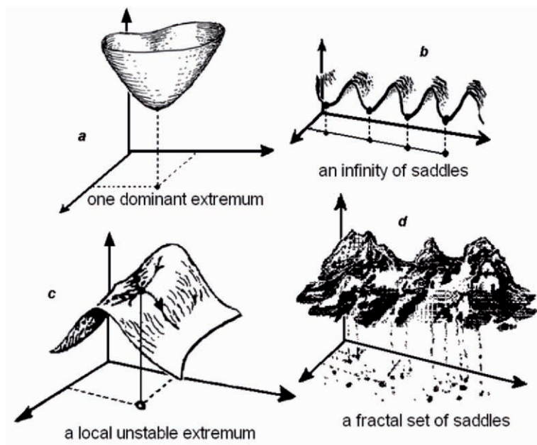
Fig. 9.1. Path integrals and chaos field theory (see text for explanation).
