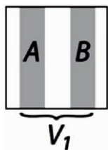
Fig. 1.25. The basic domains of the horseshoe map in symbolic dynamics.
