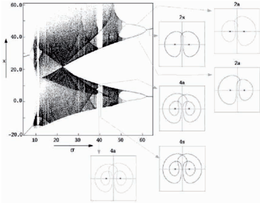
Fig. 8.1. (\sigma, x) -bifurcation diagram at fixed r = 178 , b = 8/3 for 4 < \sigma < 65 . A few periodic orbits are shown in (y, z) -projection, of periods 2 in the upper right part, and periods 4 in the lower right; arrows indicate the corresponding branches of the bifurcation diagram. The conspicuous merging of the two major chaotic bands, as \sigma is lowered, seems to occur at or very close to the value \sigma_s(r) = \sqrt{br} = 21.8 (adapted from [DSR05]).
