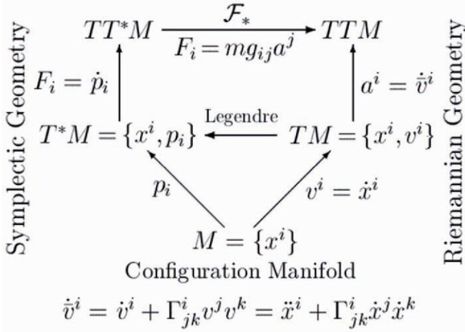
Fig. 1.55. The covariant force functor, including the main relations used by differential-geometric modelling of complex continuous systems.
