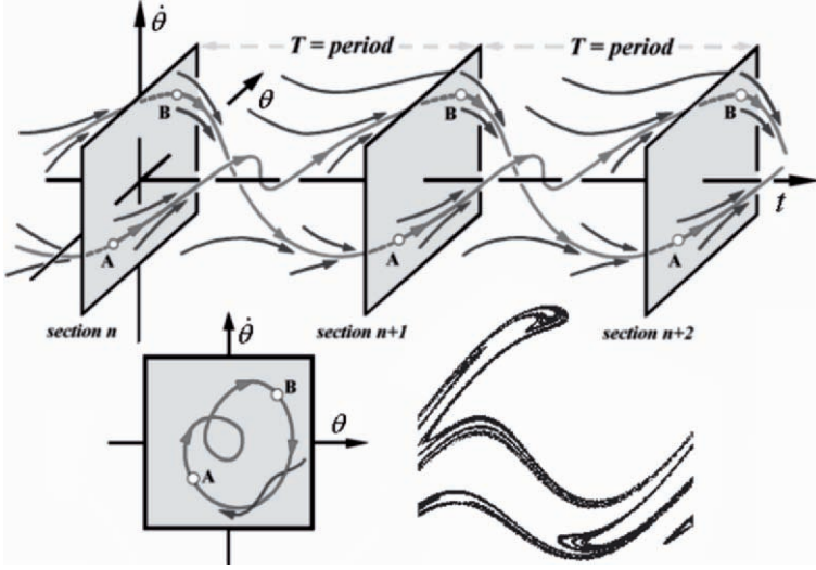
Fig. 1.39. A driven pendulum has a 3D phase-space with angle \theta , angular velocity \dot{\theta} and time t . Dashed lines denote steady states, while solid lines denote transients. Right-down we see a sample chaotic attractor (adapted and modified from [TS01]).
