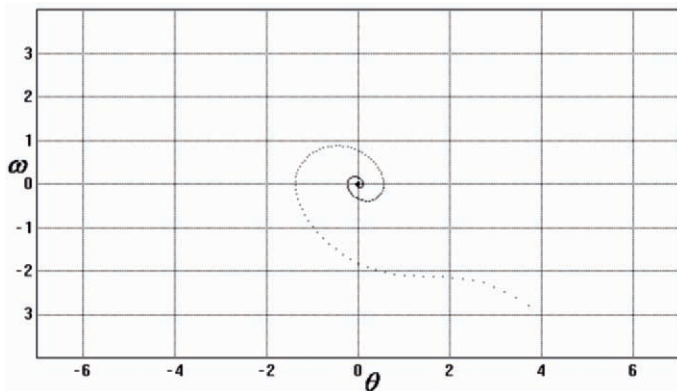
Fig. 1.2. Phase portrait of the driven nonlinear pendulum, showing the points spiralling into (0,0) .
