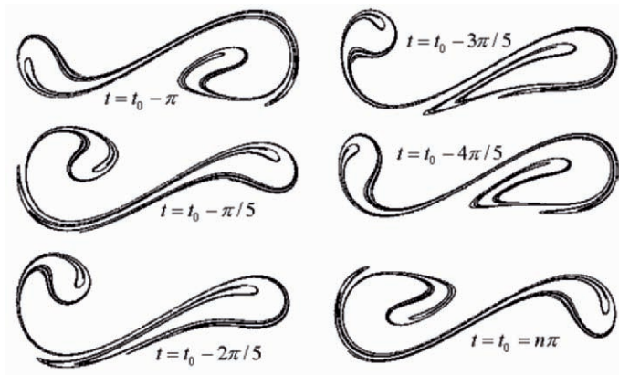
Fig. 1.41. Duffing strange attractor, showing stroboscopic Poincaré sections; simulated using Dynamics Solver TM .
