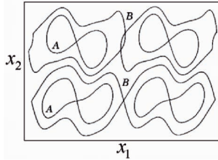
Fig. 1.56. Structure of the separatrices in the 5-mode model (1.138) with \text{Re} = \text{Re}_1 - 0.05 (adapted from [BLV01]).
