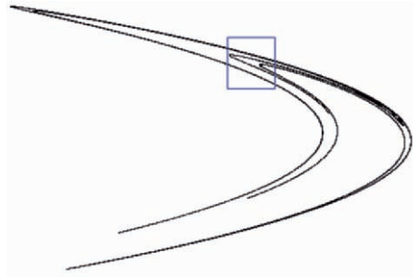
Fig. 1.32. Hénon strange attractor (see text for explanation), simulated using Dynamics Solver TM .
