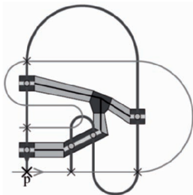
Fig. 2.7. A trellis T with its thick graph representative \hat{G} (adapted from [Col02, Col05])
