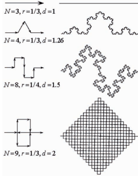
Fig. 1.49. Fractal dimension of curves in \mathbb{R}^2 : d = \frac{\log N}{\log 1/r} .
