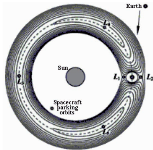
Fig. 1.19. The Lagrange's points ( L_1, \dots, L_5 ) used for the space flights. Points L_1, L_2, L_3 on the Sun–Earth axis are unstable. The SOHO spacecraft used a halo orbit around L_1 to observe the Sun. The triangular points L_4 and L_5 are often stable. A Japanese rescue mission used a chaotic Earth–Moon trajectory.
