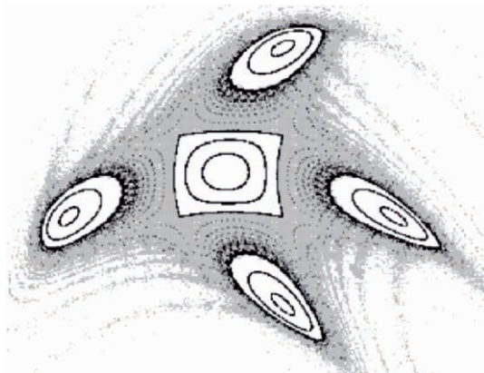
Fig. 7.4. KAM islands (blank) and stable manifold (gray; modified and adapted from [MMG05]).
