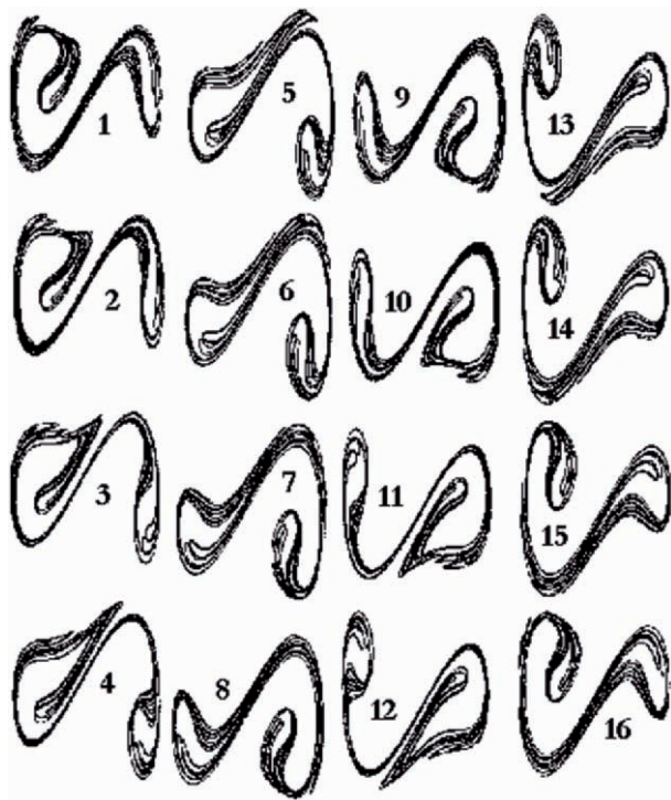
Fig. 2.1. Stroboscopic Poincaré sections (in order from 1 to 16) of a Duffing strange attractor. We can see phase-space stretching, folding and squeezing of the Duffing oscillator 1.37; simulated using Dynamics Solver TM .
