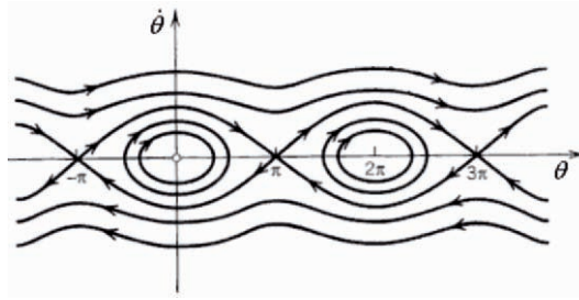
Fig. 1.37. Phase portrait of a simple gravity pendulum.
