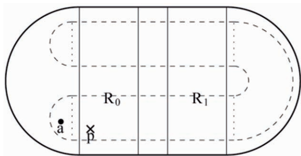
Fig. 2.2. The Smale horseshoe map.
