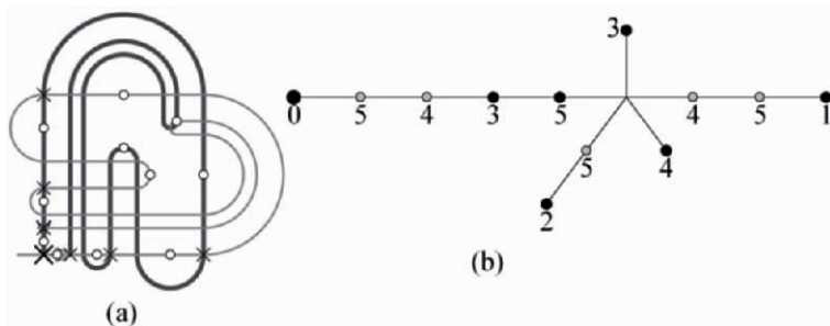
Fig. 2.6. Trellis forced by \bar{0}11111\bar{1}0 and its topological tree representative (adapted from [Col02, Col05]).
