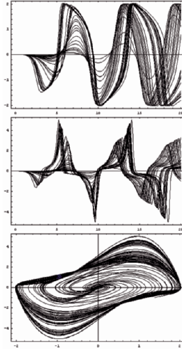
Fig. 1.40. Cascade of 30 unforced Van der Pol oscillators, simulated using Mathematica TM ; top-down: displacements, velocities and phase-plot (showing the celebrated limit cycle).
